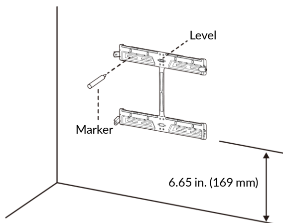
Wall mount with floor support
