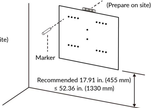
Wall mount above the floor
