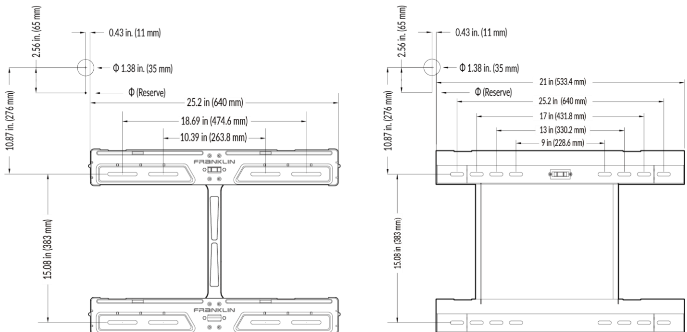
Front View: Location of bracket and conduit entry hole on the wall
